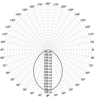
Candela Curve
