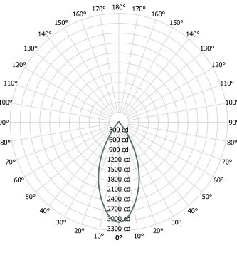
Candela Curve
