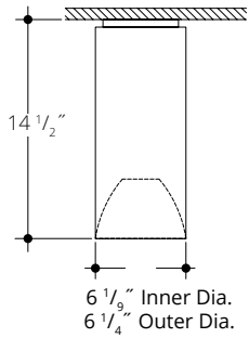
VC - CEILING/SURFACE MOUNT
