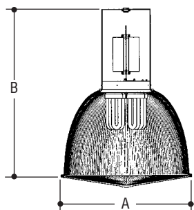
Conical Lens
