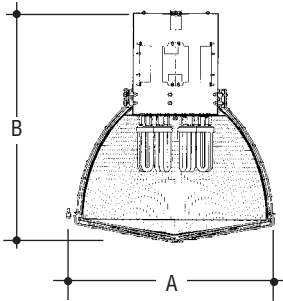
Drop Lens
